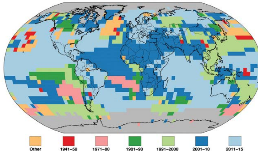
Warmest Years on Record 1880–2015 NOAA's National Centers for Environmental Information Data Source: GHCN-M version 3.3.0 & ERSST version 4.0.0
